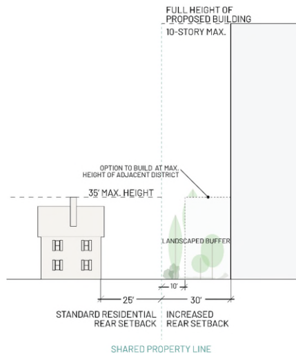
Figure 608-A. Residential Adjacency diagram
