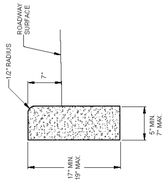
TYPICAL GRANITE CURB
